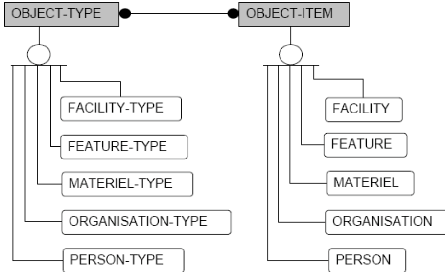
Fig 2. Conceptual relationship between OBJECT-TYPE and OBJECT-ITEM (Copied from [2])
