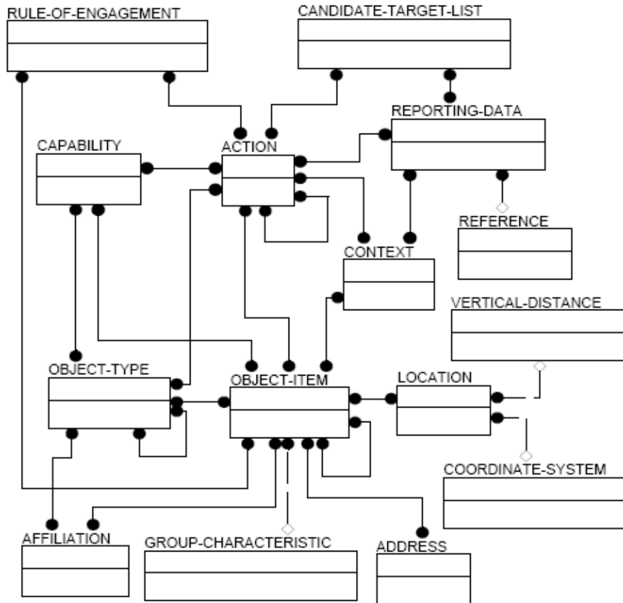
Fig 1. JC3IEDM Independent Entities. (Copied from [2])
